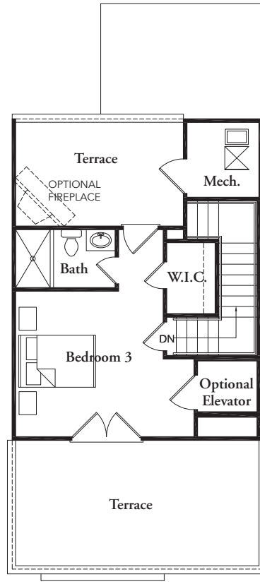
TERRACE LEVEL
