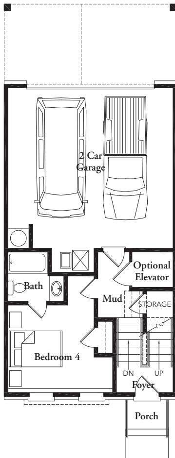
LOWER LEVEL
