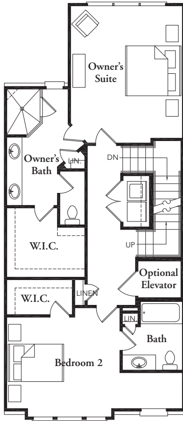
UPPER LEVEL
